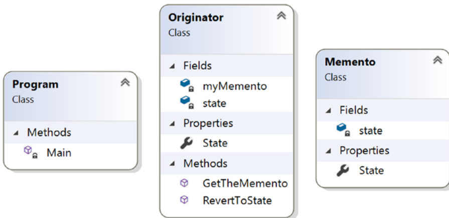
Figure 19-1. Class diagram
