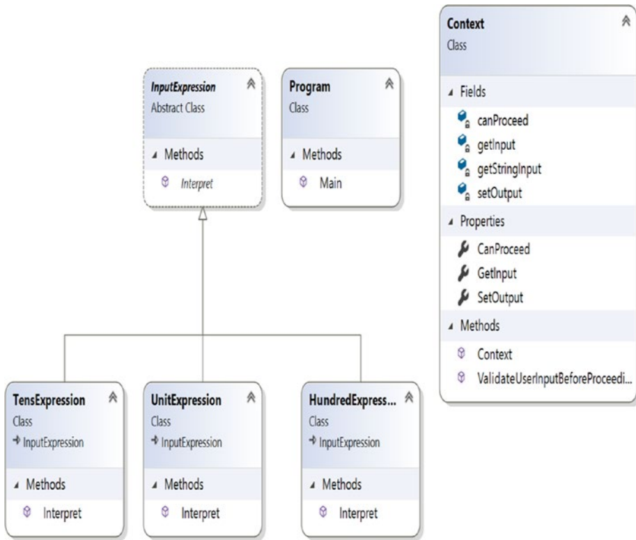
Figure 23-1. Class diagram
