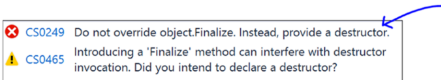
Figure 29-3. Quiz output
