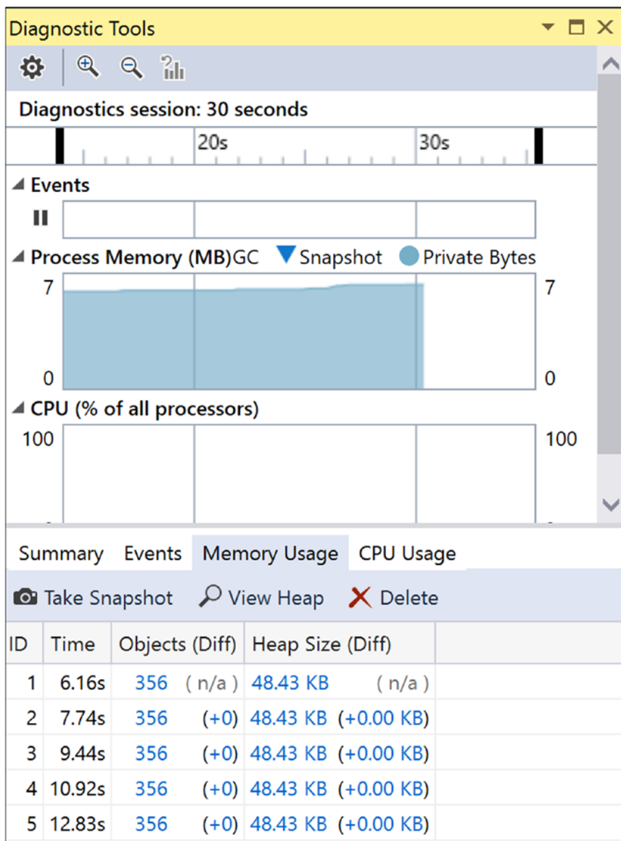
Figure 29-11. Modified results
