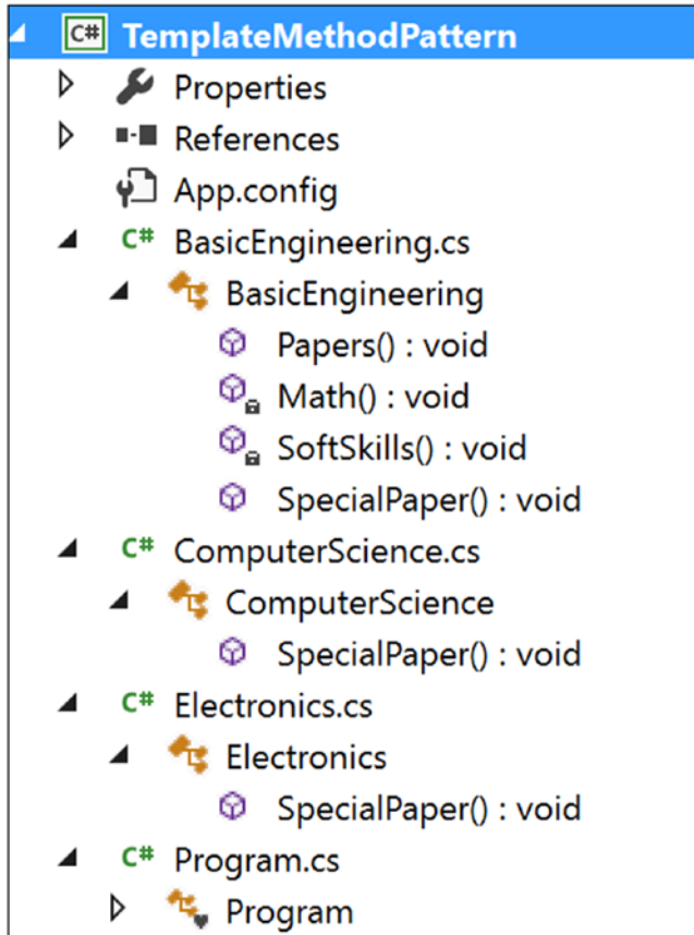
Figure 16-2. Solution Explorer View
